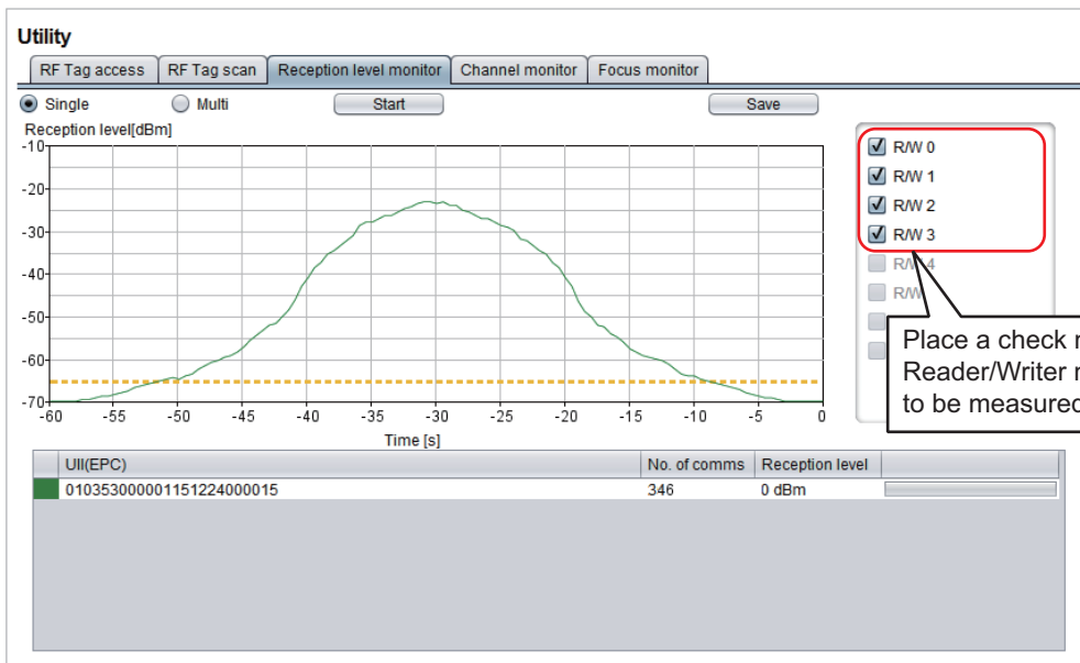
Time Series Graph of Measured Reception Level in each Reader/Writer (Can be referenced by file output)
