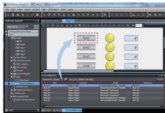
Click the location to access the object where the variable is used.
