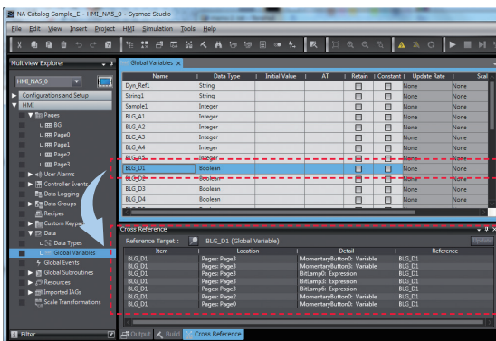
Click the variable in the global variable table to show a list of the locations where the variable is used in the Cross Reference Tab Page.
